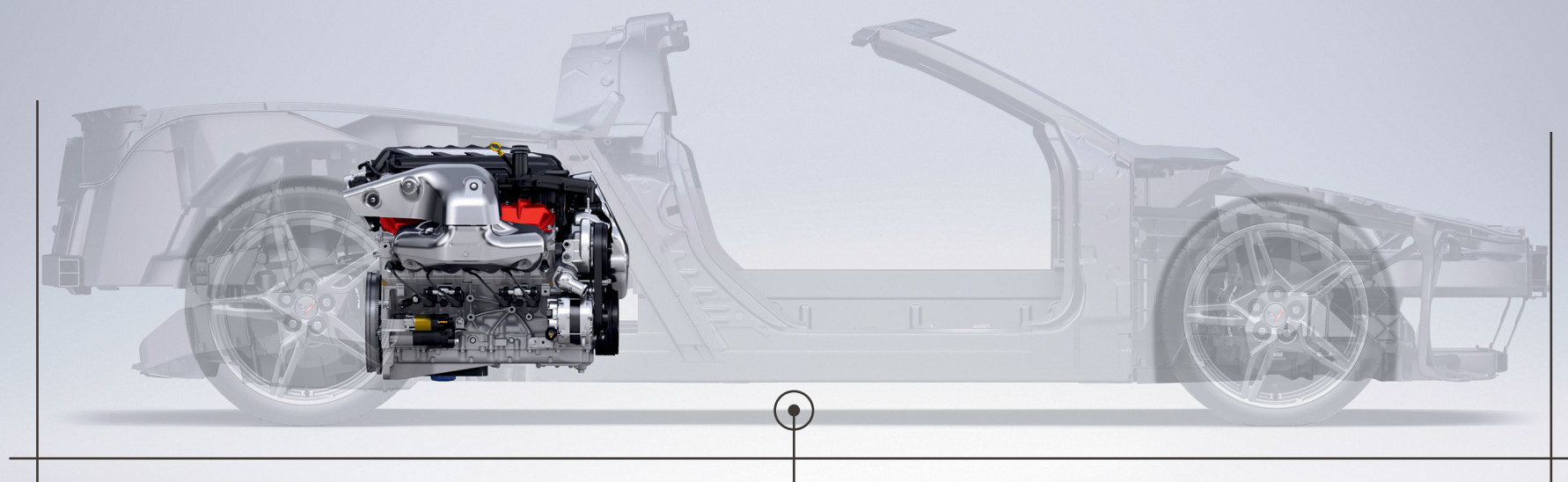
40/60 FRONT-TO-REAR WEIGHT DISTRIBUTION
